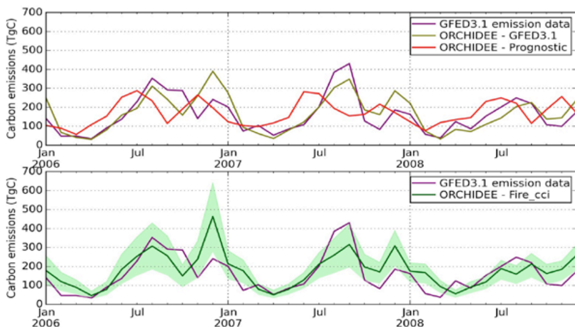
Figure 3: Global monthly fire emissions of carbon estimated with the ORCHIDEE global vegetation model using Fire_cci data from the first phase, compared to GFED 3 data. Use of Fire_cci data in global vegetation and climate models will be extended in the second phase of the project.
