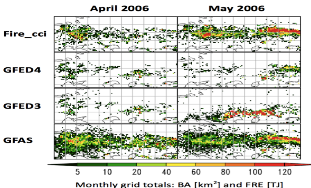
Figure 2: Burned area in Eastern Europe detected by Fire_cci, GFED4 and GFED3 in April/May 2006. GFAS shows the spatial pattern of fire radiative energy (FRE) estimated from the MODIS active fire product.
